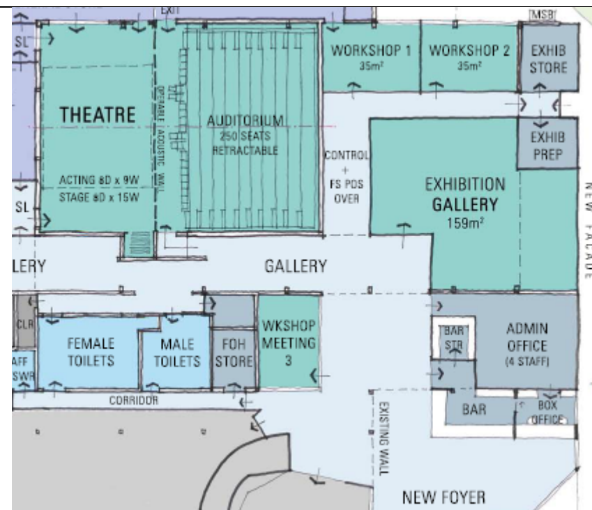
FIGURE 1 Schematic Floor Plans for remodelling of the Torquay Sports & Recreational Centre
