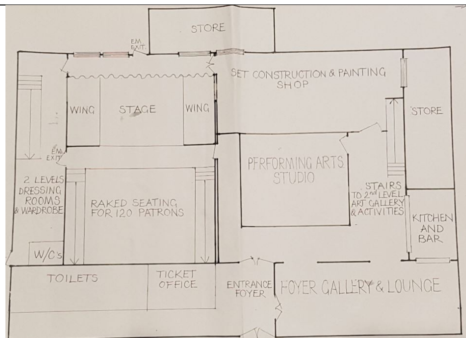
FIGURE 1 Schematic Floor Plans for remodelling of the Torquay Sports & Recreational Centre
